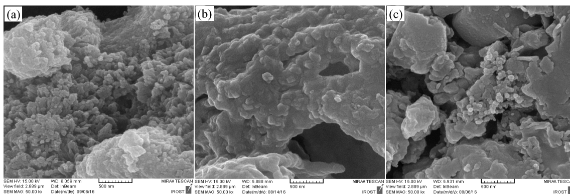
Fig. 3. SEM micrographs of the as-combusted \text{CoFe}_2\text{O}_4 powders using (a) urea, (b) glycine and (c) citric acid fuels
