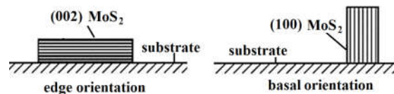
Fig. 9. Two categories of MoS 2 coatings in terms of crystallographic orientations.
