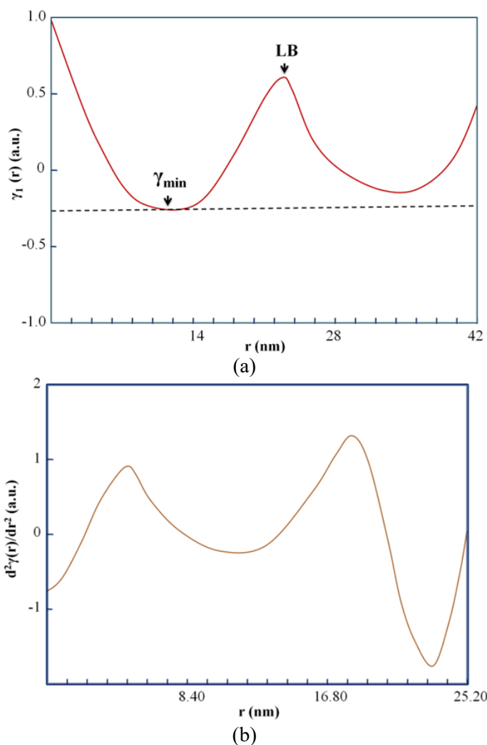
Fig. S1. 1D correlation function ( \gamma_1(r) ) (a) and of IDF (b) of SAXS of PEG5000-b-PCL9100 single crystals grown at T_c=28^\circ\text{C} .
