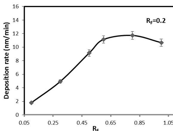
Fig. 2. Deposition rate of a-CN x as a function of R F
