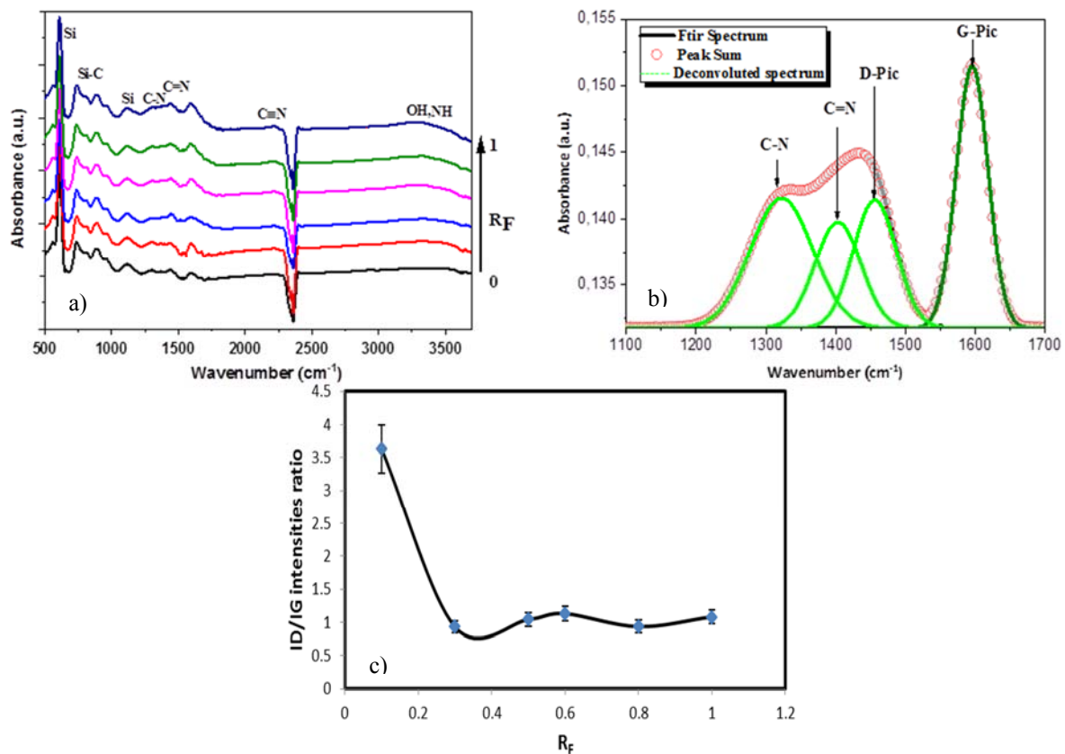
Fig. 6. a) FTIR absorption spectra of a-CN x thin films for different R F values b) Deconvolution of FTIR absorption spectrum of a-CN x thin films in 1200-1700 cm -1 zone for R F = 1 c) (I_D/I_G) intensities ratio of the Infrared D and G bands of the a-CN x thin films as a function of different values of R F .
