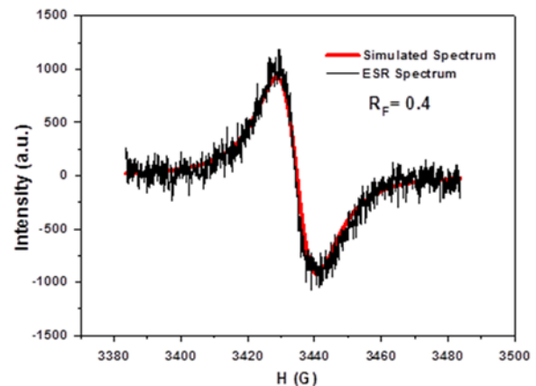
Fig. 4. ESR spectra of a-CN x thin films for R_F=0.4 owing
