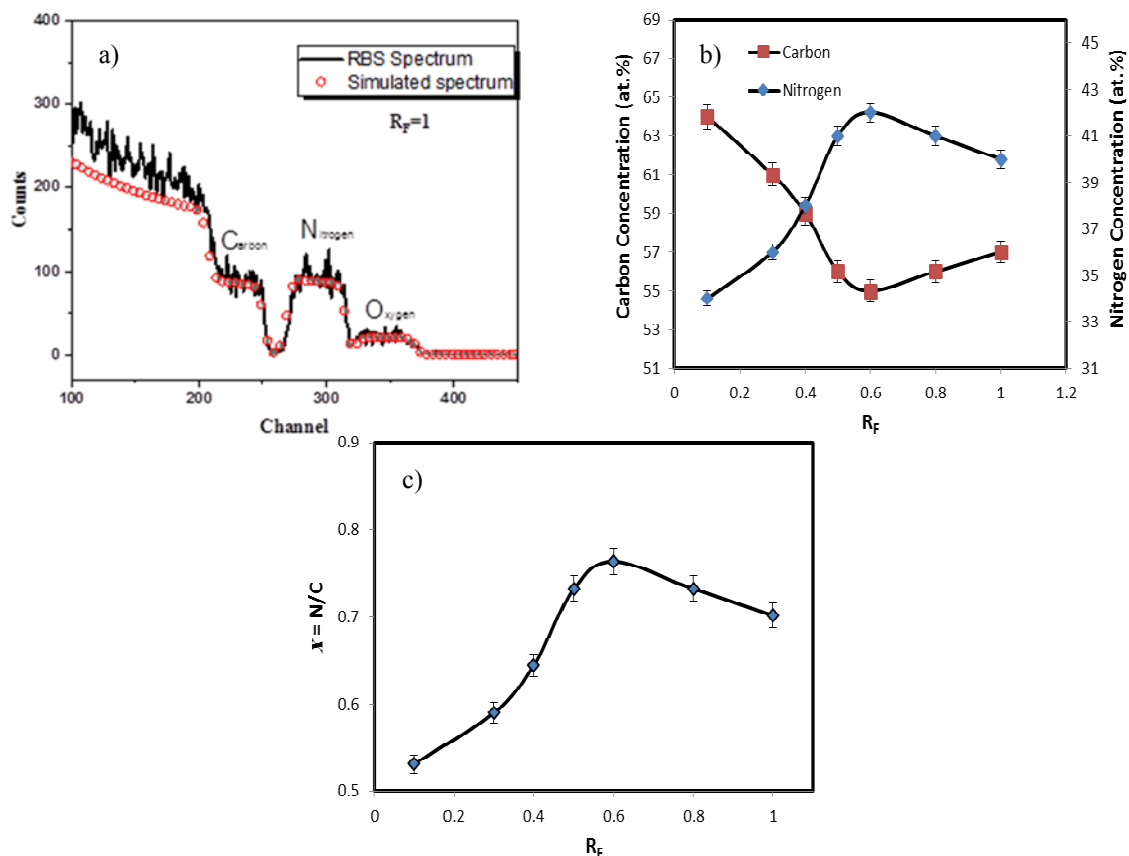
Fig. 3. a) Experimental and simulated RBS spectrum for R_F=1 b) Composition of a- CN_x films as a function of R_F c) Ratio of the number of nitrogen and carbon atoms in a- CN_x films.
