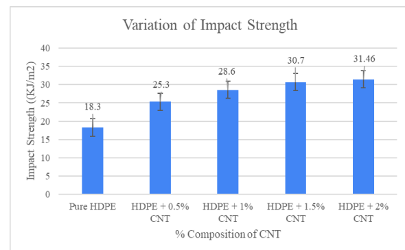
Fig. 5. Variation of Impact strength of HDPE with CNT reinforcement
