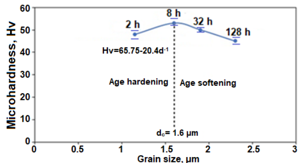
Fig. 14. Relationship between the hardness and the grain size of Zn-22Al alloy after post-ECAP aging at 250°C.
