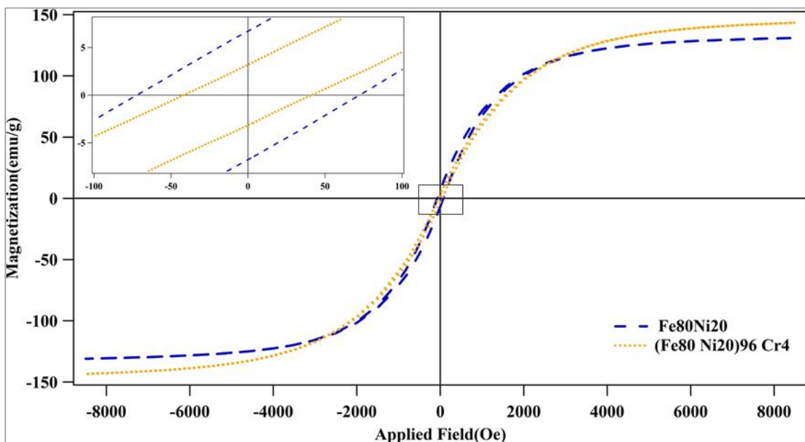
Fig. 15. Magnetization versus applied magnetic field for Fe_{80}Ni_{20} and (Fe_{80}Ni_{20})_{96}Cr_4 milled for 96 hours
