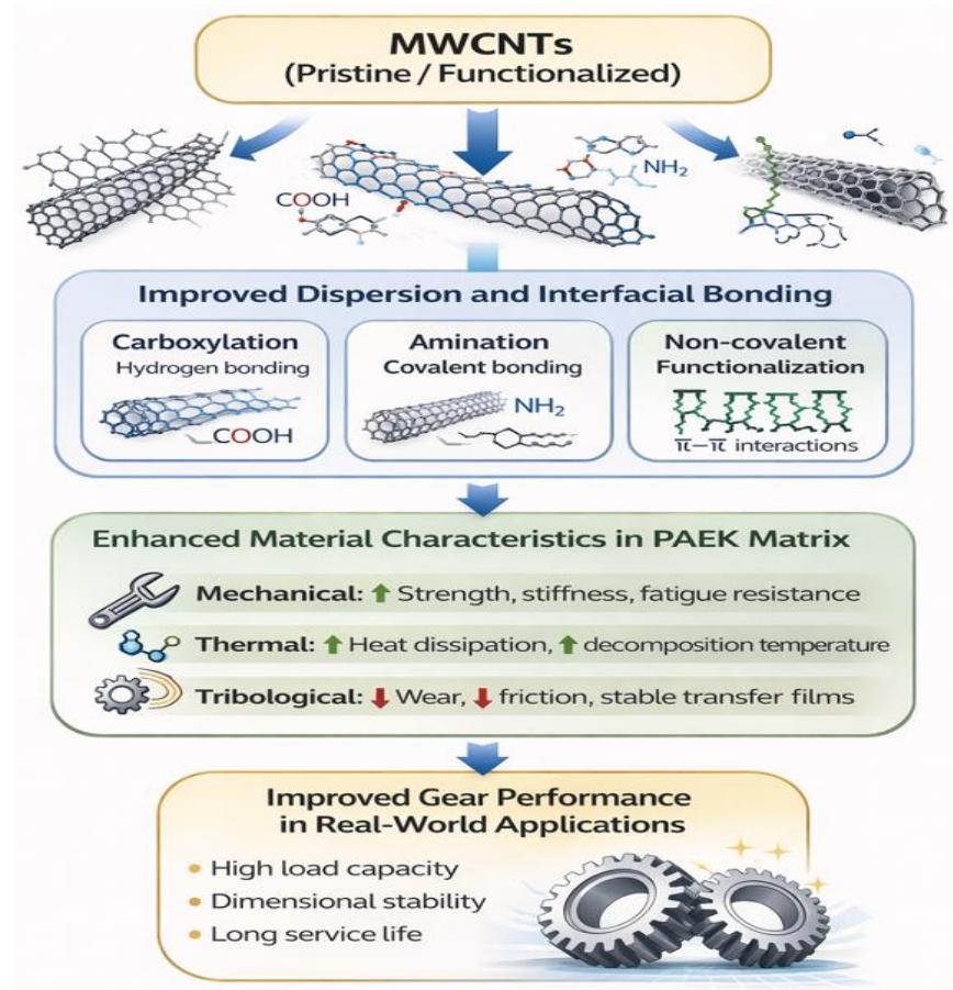
Figure 1. Conceptual diagram illustrating reinforcement mechanisms of MWCNTs in PAEK composites for gear applications.
