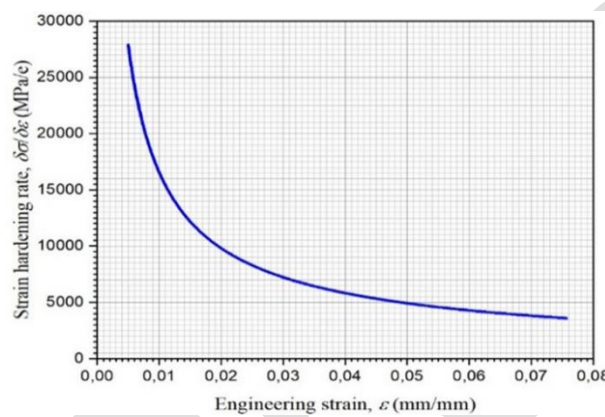
Fig. 4. The relationship between strain hardening rate and engineering strain
