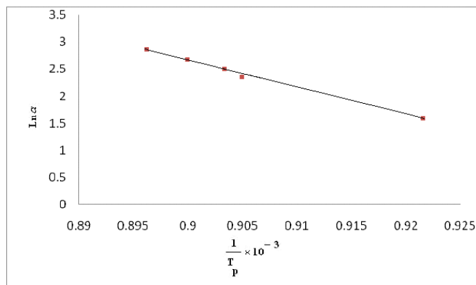
Fig 8. Variation of Ln vs \alpha in ST_3Z_1Y_1 for determination of the crystallization activation energy according to Marotta method
