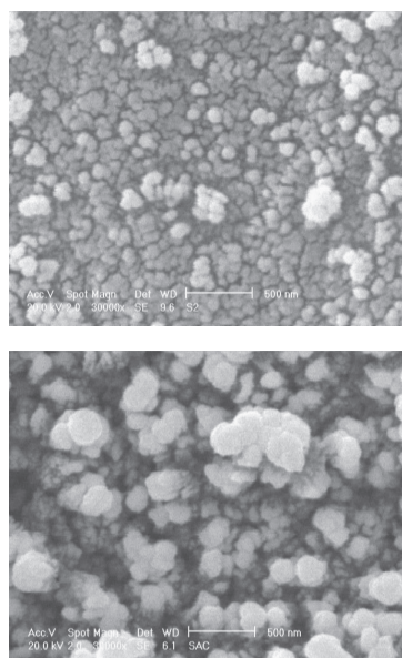
Fig. 5. SEM images of prepared pure TiO 2 (a) and nitrogen doped TiO 2 (b) nanoparticles.
