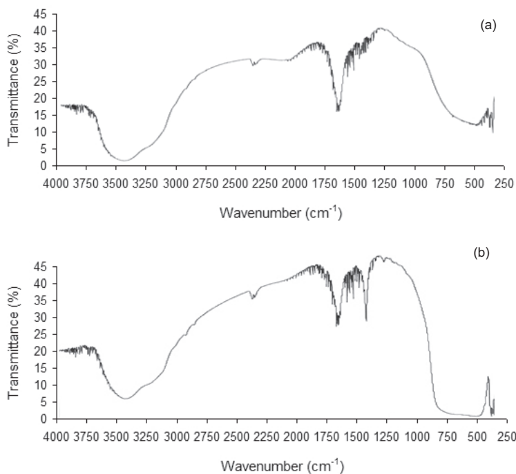
Fig. 3. FTIR spectra of prepared pure TiO 2 (a) and nitrogen doped TiO 2 (b) samples.
