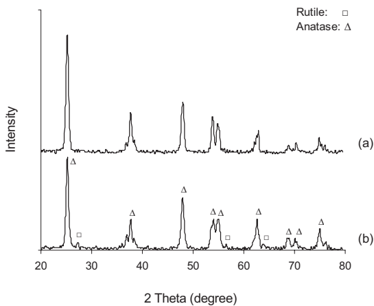
Fig. 4. XRD patterns of prepared nitrogen doped TiO 2 (a) and pure TiO 2 (b).
