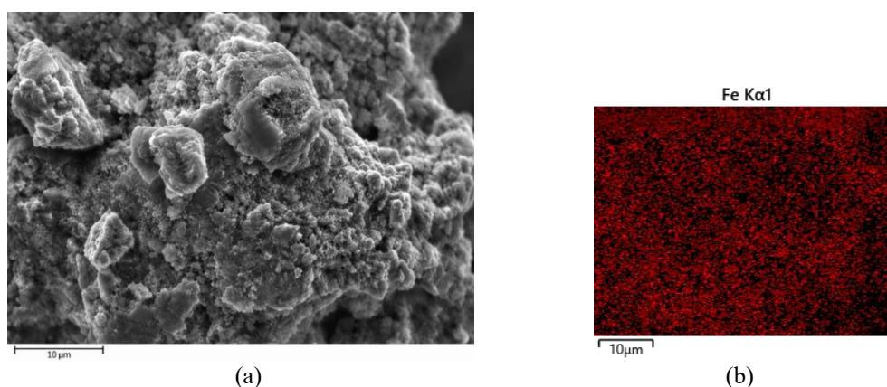
Fig. 3. a) SEM morphology at 7 \text{ A dm}^{-2} , b) EDX Fe map showing uniform Fe distribution at 7 \text{ A dm}^{-2}
