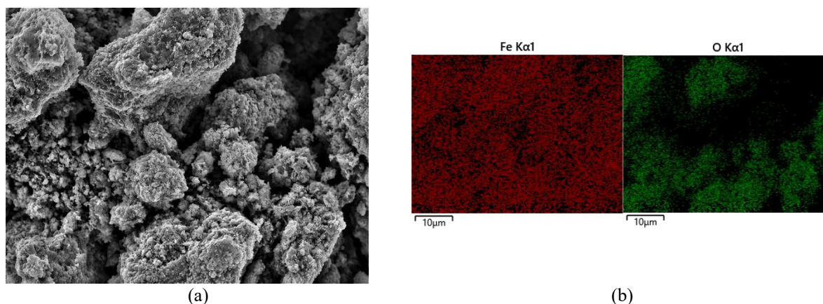
Fig. 4. a) SEM morphology at 10 \text{ A dm}^{-2} , b) EDX. Fe and O maps of the 10 \text{ A dm}^{-2} powder
