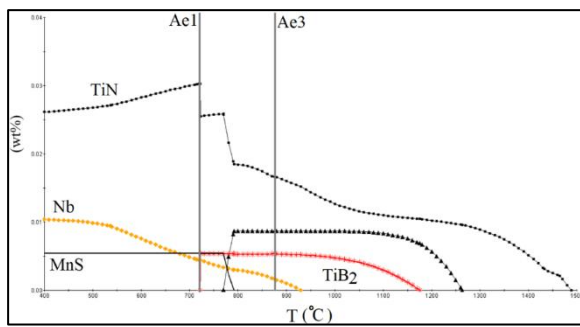
Fig. 12. Thermodynamic analysis of potential precipitates in the FBT sample
