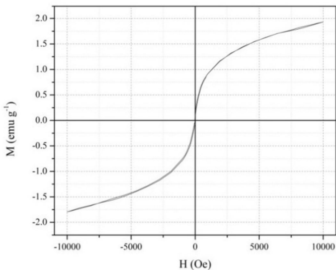
Fig. 3. Hystersis loop of sample glass.
