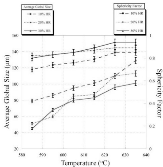
Fig. 7. Variations of average grain size and sphericity factor in Ti-refined Al2014 alloy with 10, 20 and 30% HR, versus holding temperature in semi solid state for 30 min.
