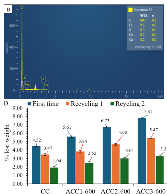
Fig. 10. A) FTIR transmission spectra of fresh ACC3-600 and reused ACC3-600 after recycling two times, B) EDS of reused ACC3-600 after recycling two times, C) SEM of reused ACC3-600 after recycling two times, D) percent weight loss of CC and ACCs after oxidation conversion at first time, first recycling, and second recycling (the error bars represent standard deviation)
