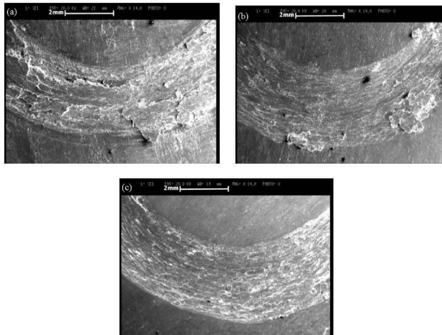
Fig. 5. The SEM images of the surface of worn nanocomposite with (a) 0.5, (b) 1 and (c) 2Wt% nano SiO 2 at 8th cycle of ARB process
